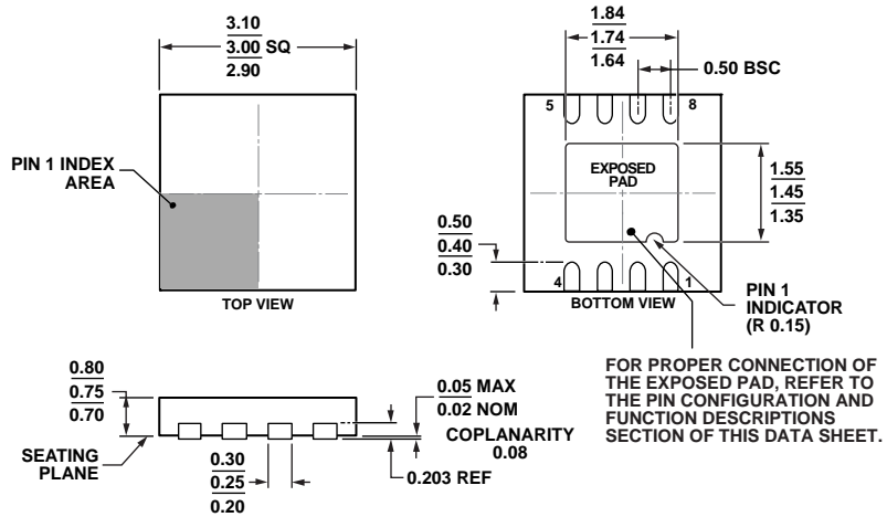
Figure 27. 8-Lead Lead Frame Chip Scale Package [LFCSP_WD] 3 mm x 3 mm Body, Very Very Thin, Dual Lead (CP-8-13) Dimensions shown in millimeters
