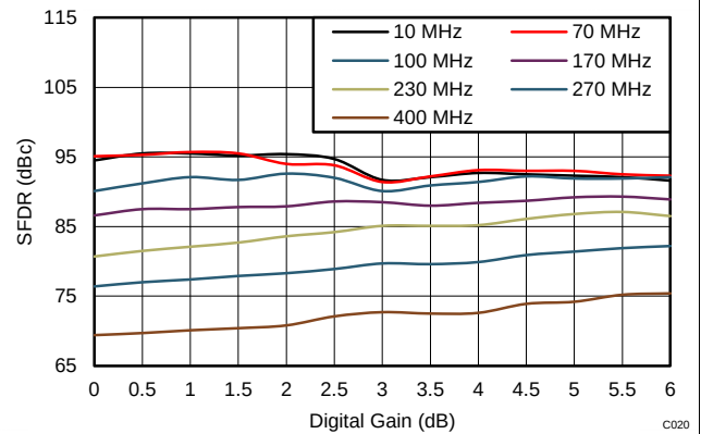
Figure 86. Spurious-Free Dynamic Range vs Digital Gain and Input Frequency
