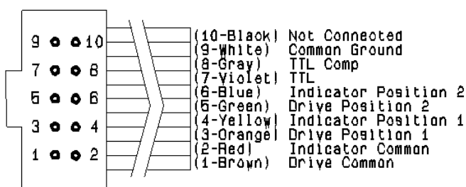
Switch connector
