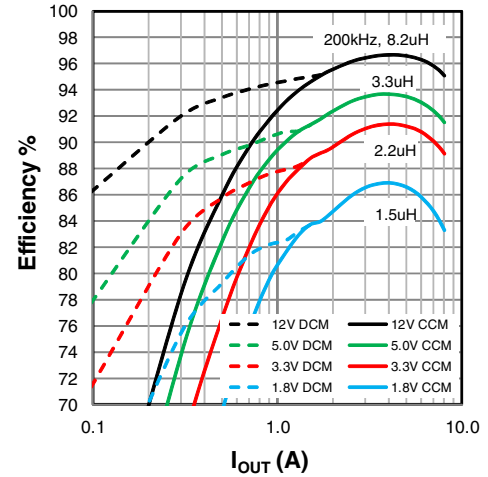
Figure 20: XR76208 efficiency, V_{\text{IN}}=24\text{V}
