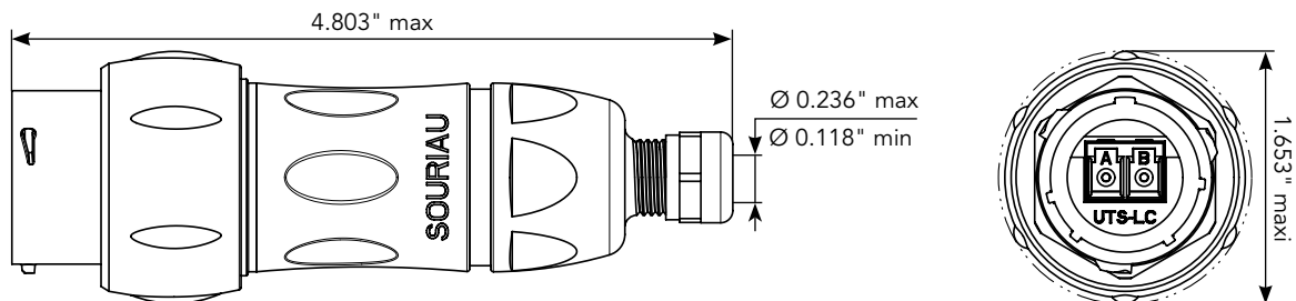
Free Hanging Receptacle -UTS1JC18LCN
