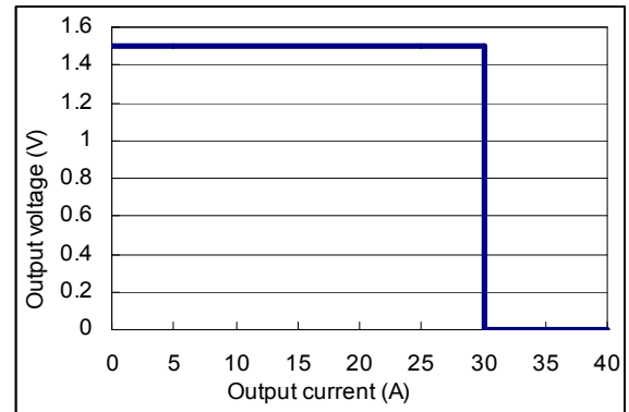
Fig.9 Typical output over-current of AVO50-48S1V5
