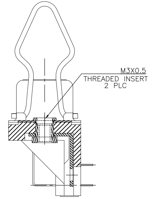
SECTION F-F
