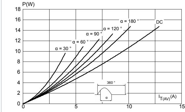
Figure 1. Maximum power dissipation versus average on-state current
