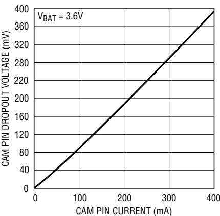
LTC3209-1 CAM Pin Dropout Voltage vs CAM Pin Current
