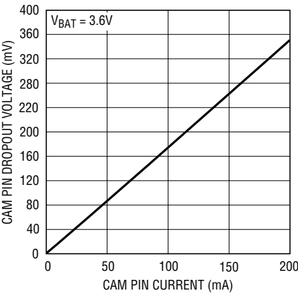
LTC3209-2 CAM Pin Dropout Voltage vs CAM Pin Current
