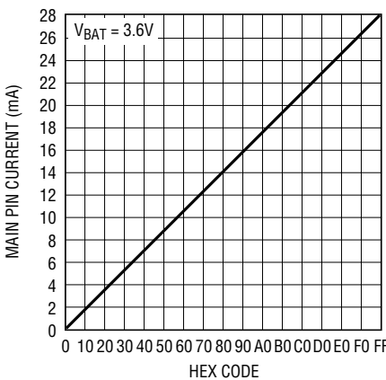
MAIN Pin Current vs Input Code
