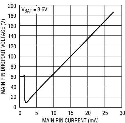
MAIN Pin Dropout Voltage vs MAIN Pin Current
