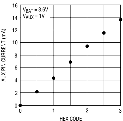
AUX Pin Current vs Input Code
