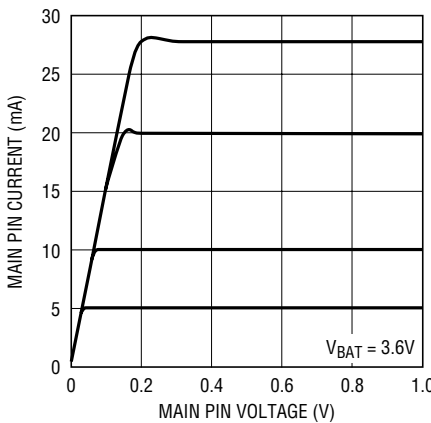
MAIN Pin Current vs MAIN Pin Voltage
