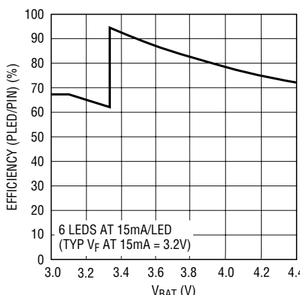
6-LED MAIN Display Efficiency vs V_{BAT}
