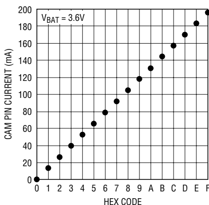
LTC3209-2 CAM Pin Current vs Input Code
