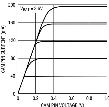
LTC3209-2 CAM Pin Current vs CAM Pin Voltage
