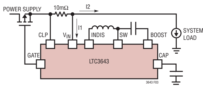
Figure 3. PowerPath of Boost Regulator with CLP Programmability
