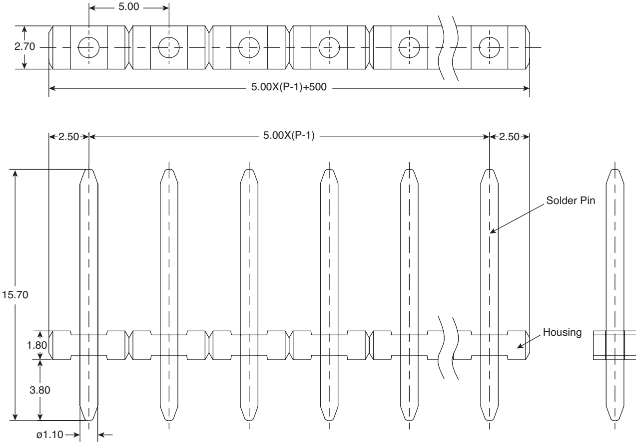
Dimensions: mm
