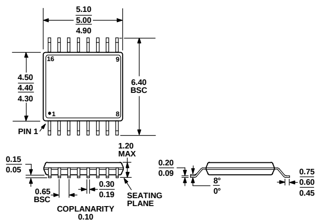
Figure 37. 16-Lead Thin Shrink Small Outline Package [TSSOP]
