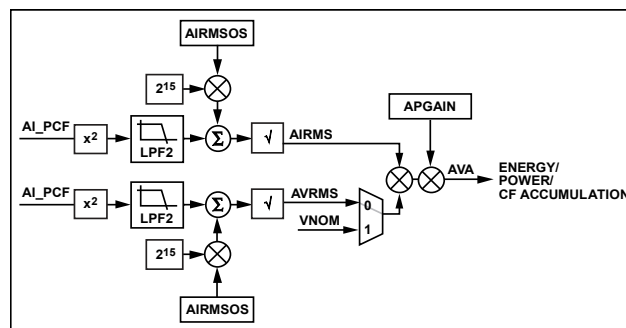
Figure 58. Total Apparent Power (AVA) Calculation
