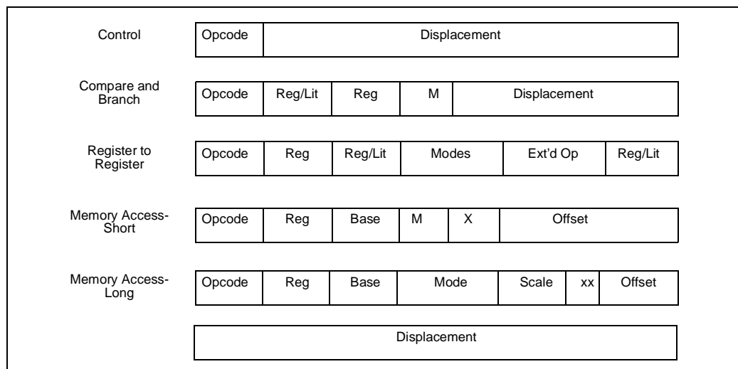
Figure 2. Instruction Formats
