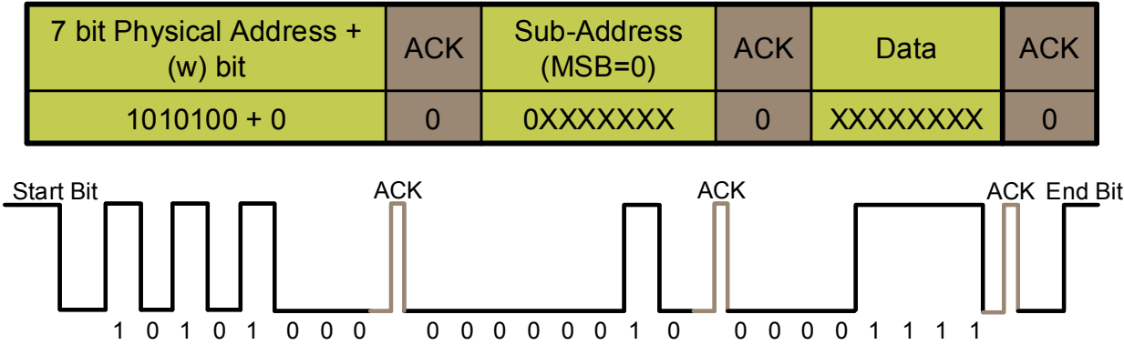
Figure 7. Writing sequence I 2 C bit stream
