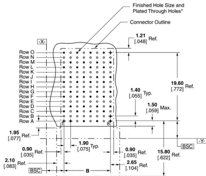
* Finished Hole Diameter = 0.46 \pm^{+0.05}_{-0.002} [0.018 \pm^{+0.002}_{-0.001} ] Drilled Hole Diameter = 0.55 \pm^{+0.02}_{-0.001} [0.022 \pm^{+0.001}_{-0.0005} ] Copper Thickness = 0.038 \pm^{+0.013}_{-0.0005} [0.0015 \pm^{+0.0005}_{-0.0002} ] Tin-Lead Thickness = 0.008 \pm^{+0.004}_{-0.0003} [0.0003 \pm^{+0.0002}_{-0.0002} ] Finishes other than Tin-Lead, See App. Spec. 114-13202
