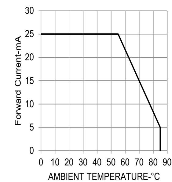
Figure 10: Derating Curve
