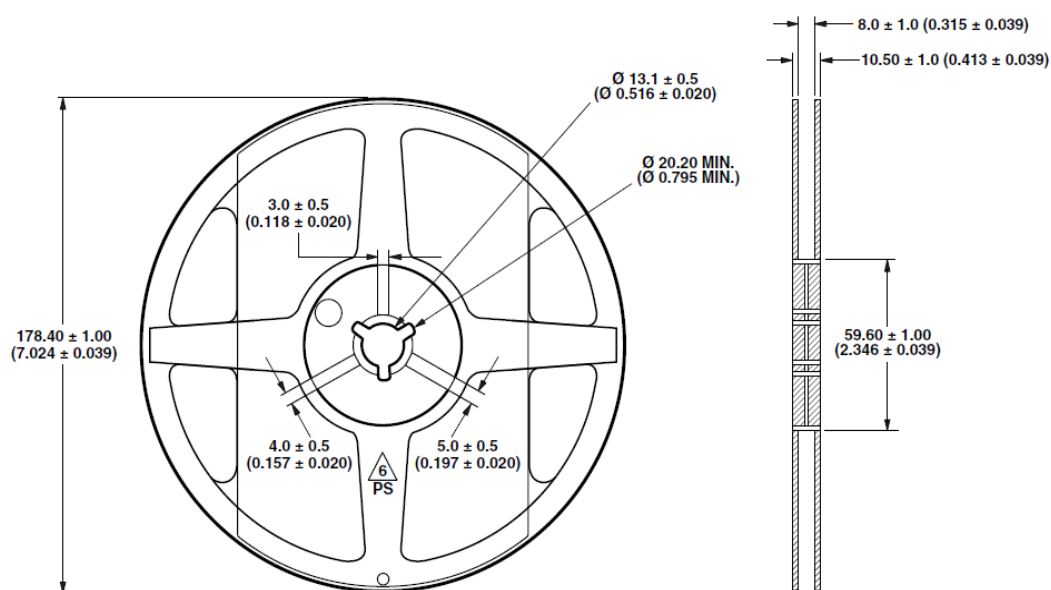
Figure 13: Reel Dimensions
