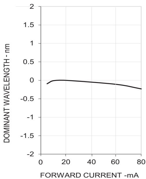
Figure 6: Wavelength Shift vs. Forward Current
