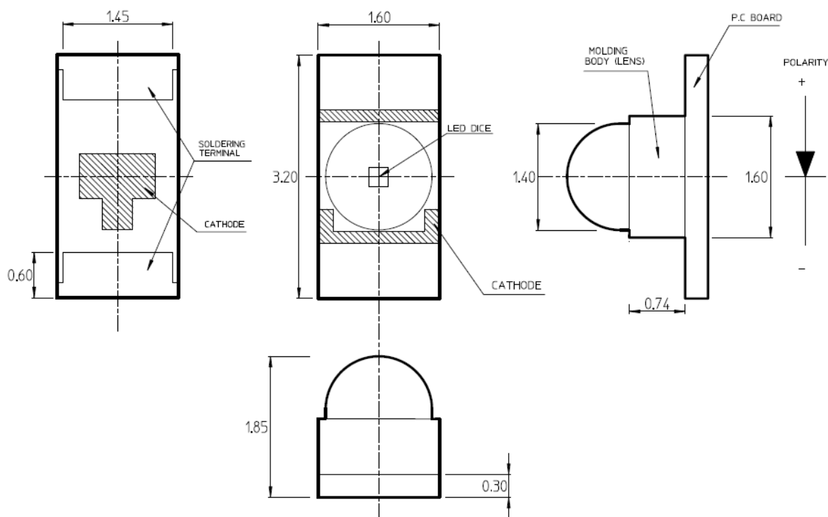
Figure 1: Package Dimensions
