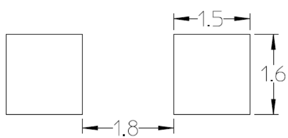
Figure 11: Recommended Solder Pad (Units: mm)
