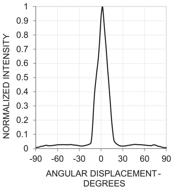
Figure 5: Radiation Pattern
