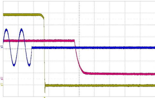
Figure 9. Turn-Off AC Line 230VAC, full load (20ms/div) CH1: V 1 (2V/div) CH2: V SB (2V/div) CH3: I in (200V/div)
