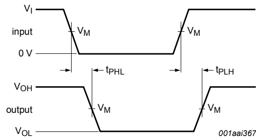
Fig. 8. The data input (nA or nBn) to output (nBn or nA) propagation delays
