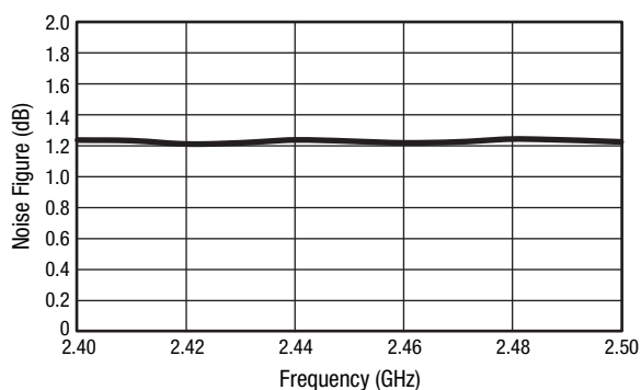
Figure 7. Noise Figure vs Frequency
