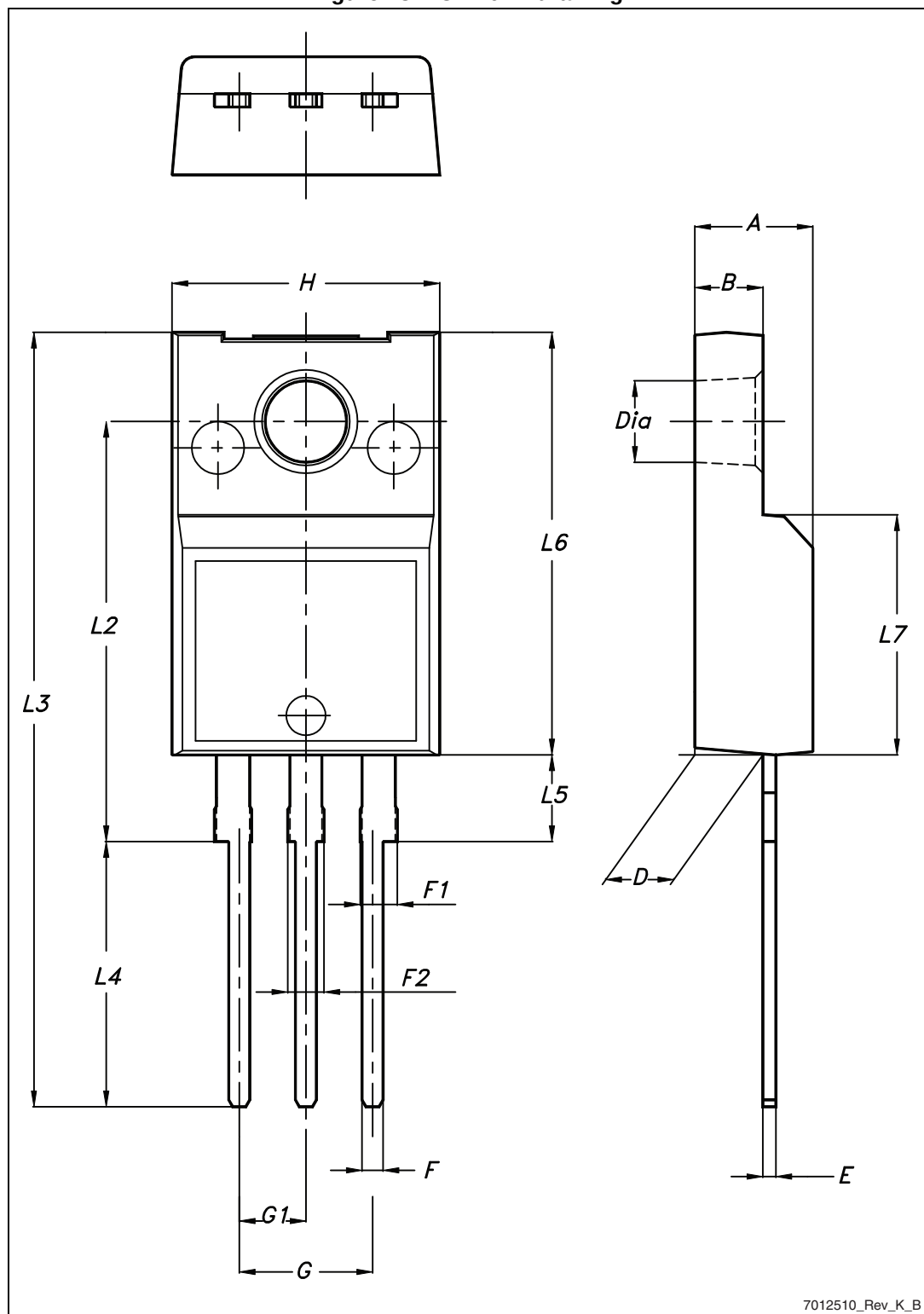
Figure 28. TO-220FP drawing
