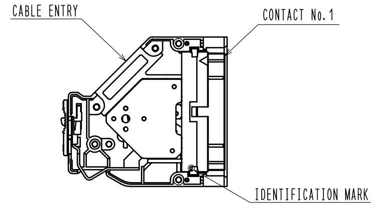
3 FIG. 1 ASSEMBLY DRAWING (1:2)
