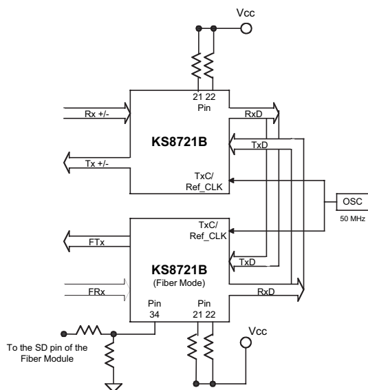
Figure 3. Fiber Module
