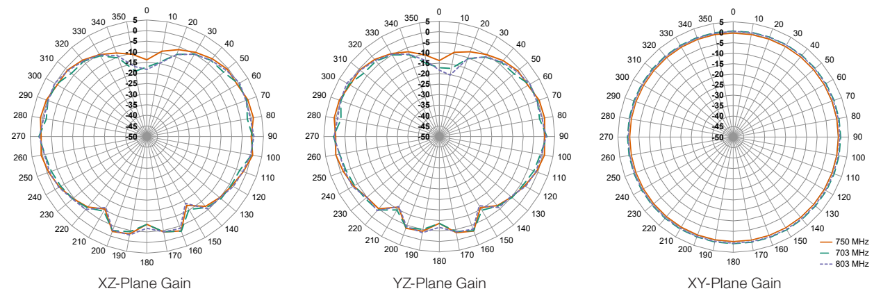
Figure8. Radiation Patterns for CW LTE Band 28 Antenna
