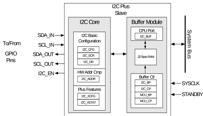
Figure 4. I 2 C Block Diagram
