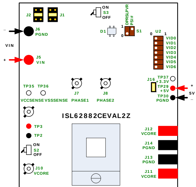
FIGURE 1. TEST SET-UP
