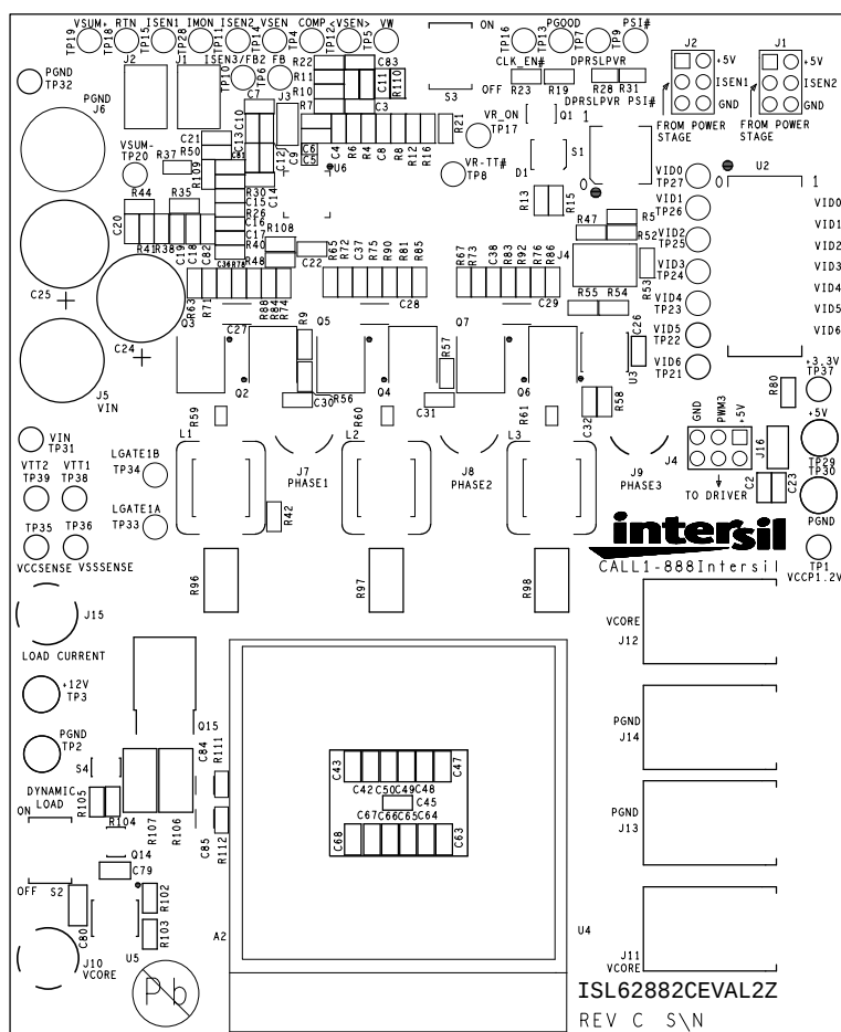
FIGURE 7. TOP SILKSCREEN
