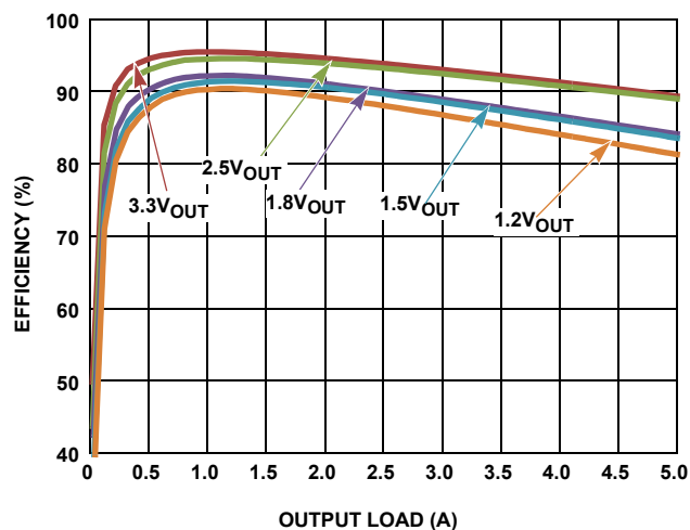
FIGURE 7. EFFICIENCY vs LOAD ( 5\text{V}_{IN} ; \text{SYNC} = V_{DD} )
