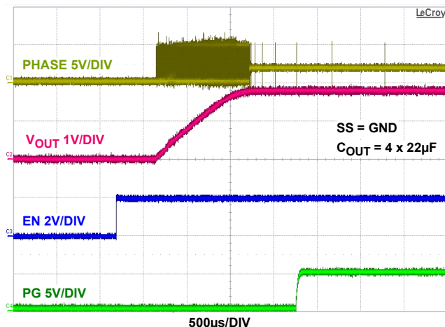
FIGURE 15. EN START-UP AT NO LOAD ( SYNC = \text{GND} )
