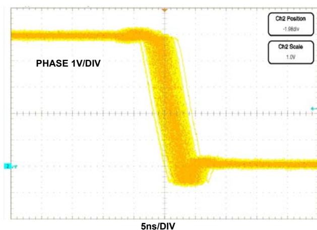
FIGURE 29. JITTER AT NO LOAD ( SYNC = V_{DD} )
