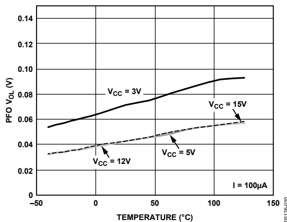
Figure 36. PFO Output Low Voltage vs. Temperature, I = 100\mu\text{A}
