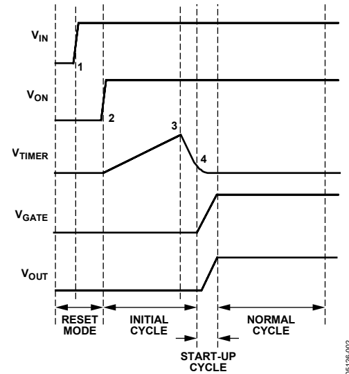
Figure 38. Power-Up Timing
