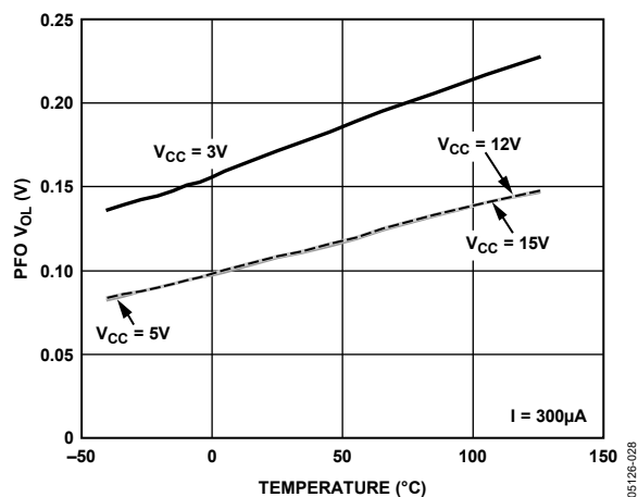
Figure 34. PFO Output Low Voltage vs. Temperature, I = 300\mu\text{A}
