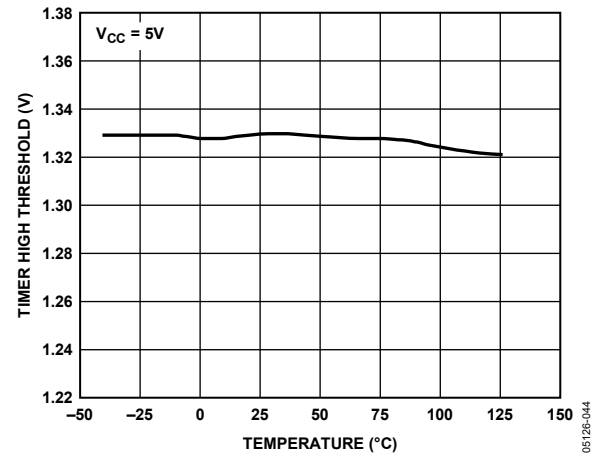
Figure 19. TIMER High Threshold vs. Temperature
