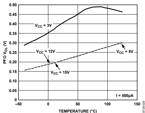
Figure 35. PFO Output Low Voltage vs. Temperature, I = 500\mu\text{A}
