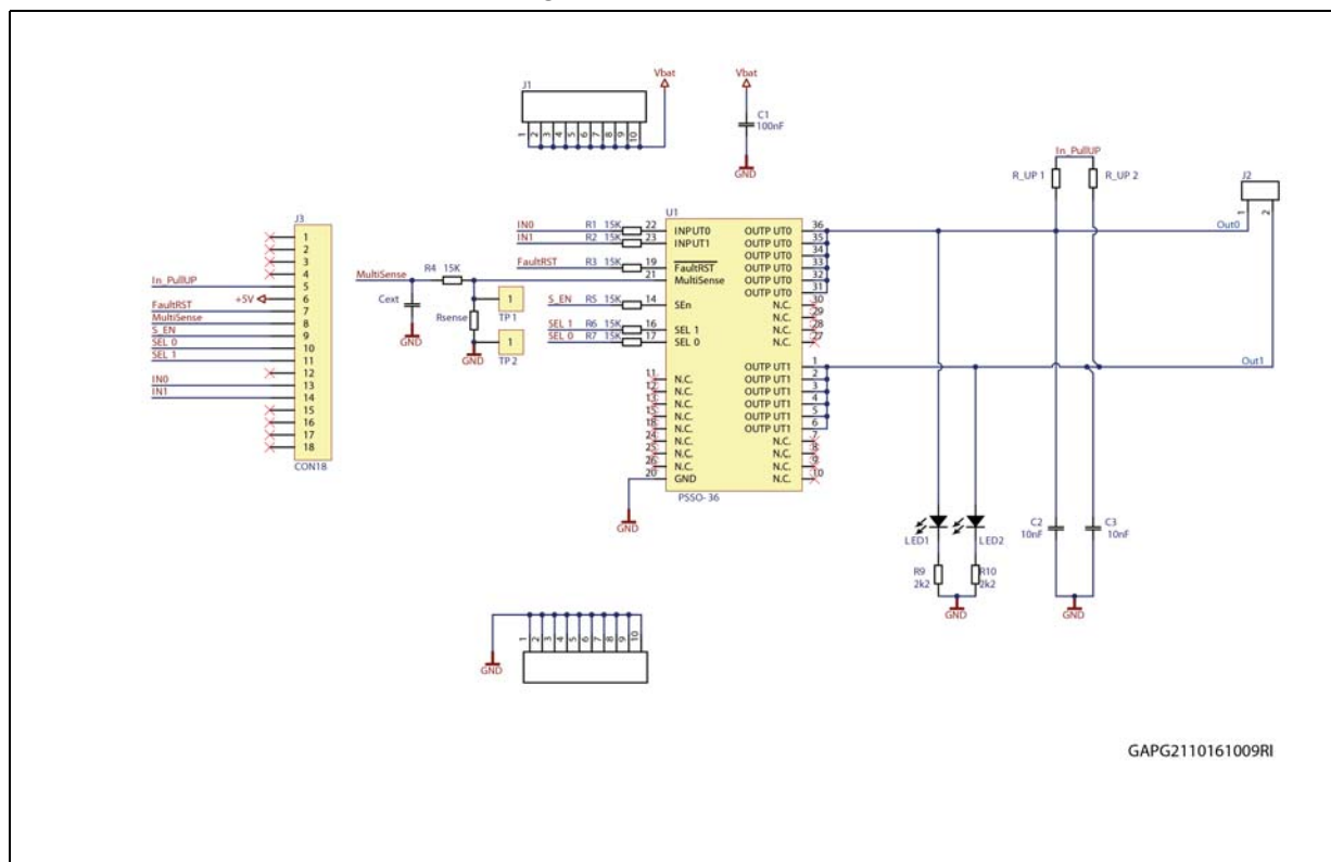
Figure 1. EV-VND7004AY schematic
