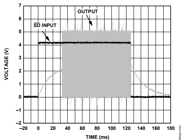
Figure 31. Turn-Off Response
