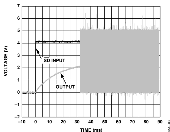
Figure 30. Turn-On Response
