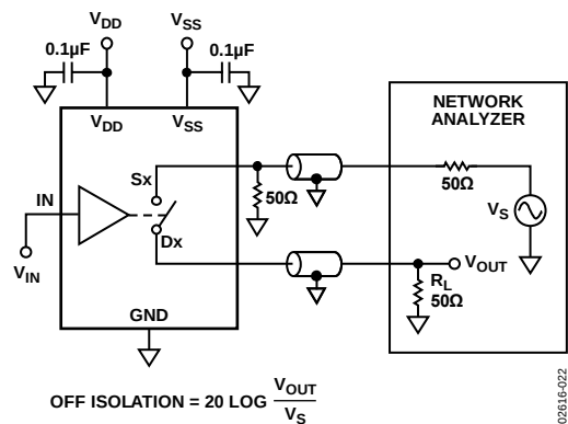
Figure 19. Off Isolation
