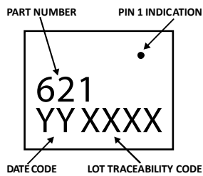
Figure 21. Package Marking Specification (Top View)
