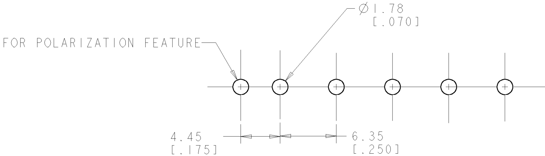
RECOMMENDED MOUNTING HOLE PATTERN FOR 1.57 [1.062] THICK P.C. BOARD
