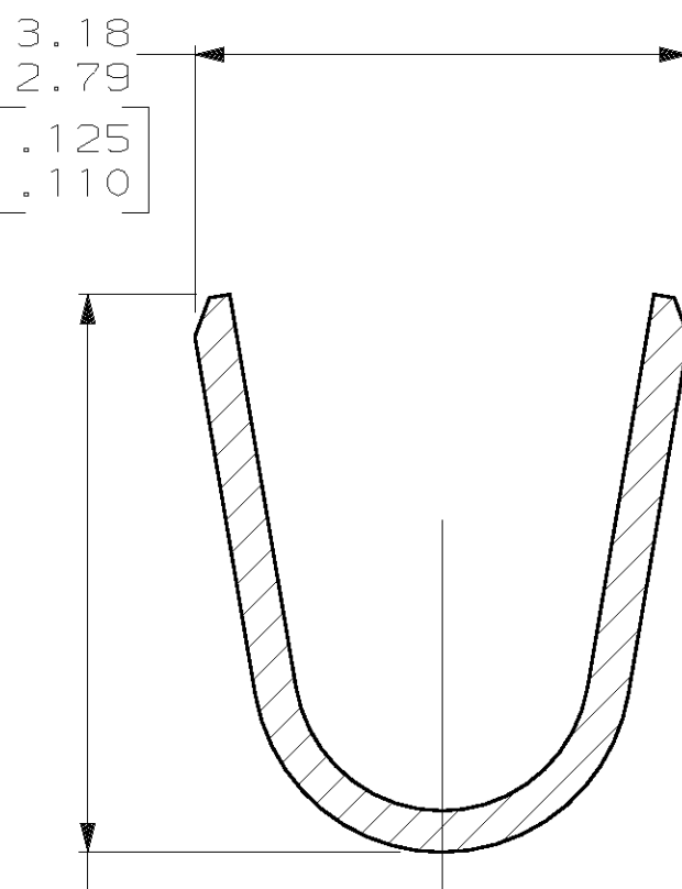
SECTION C-C SCALE 10:1
