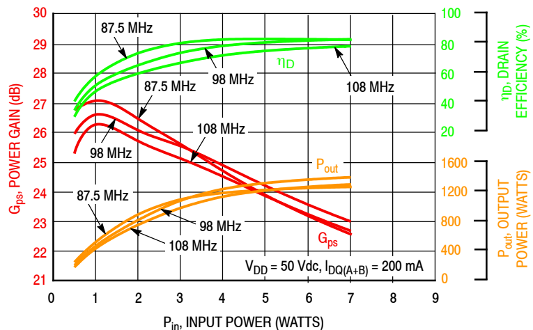
Figure 9. Power Gain, Drain Efficiency and CW Output Power versus Input Power and Frequency
