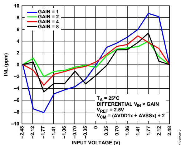
Figure 12. INL vs. Input Voltage and PGA Gain at 16 kSPS, Low Power Mode
