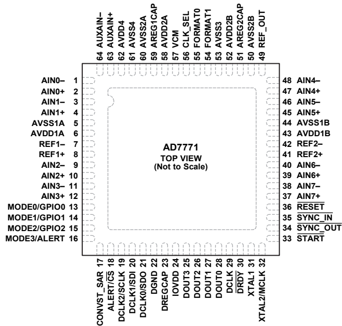
Figure 7. Pin Configuration
