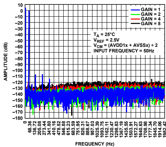
Figure 35. FFT Plot, Low Power Mode at 4 kSPS, Input Frequency ( f_{IN} ) = 50 Hz, Sinc3 Filter Enabled
