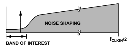
Figure 99. \Sigma - \Delta ADC Operation, Majority of Noise Energy Shifted Out of the Band of Interest (Linear Scale X-Axis)
