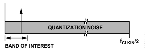
Figure 98. \Sigma - \Delta ADC Operation, Reduction of Noise Energy Contained in the Band of Interest (Linear Scale X-Axis)
