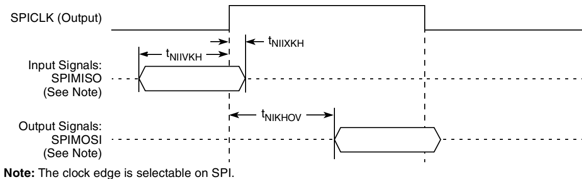
Figure 32. SPI AC Timing in Master Mode (Internal Clock) Diagram
