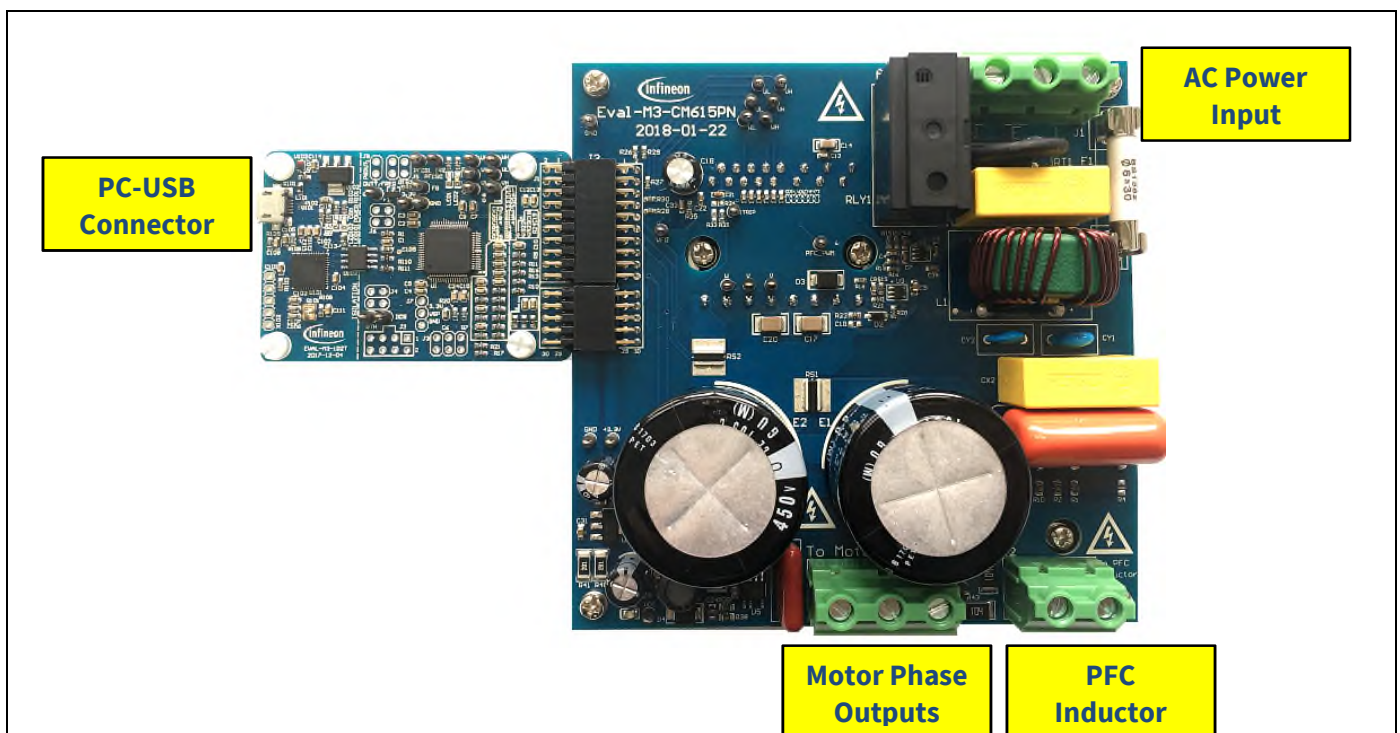
Figure 5 System connection example using EVAL-M3-102T and EVAL-M3-CM615PN
