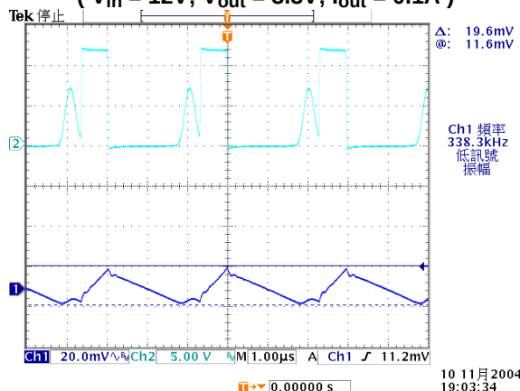
AP1513 V_{out} Ripple ( V_{in} = 12V ; V_{out} = 3.3V ; I_{out} = 0.1A )
