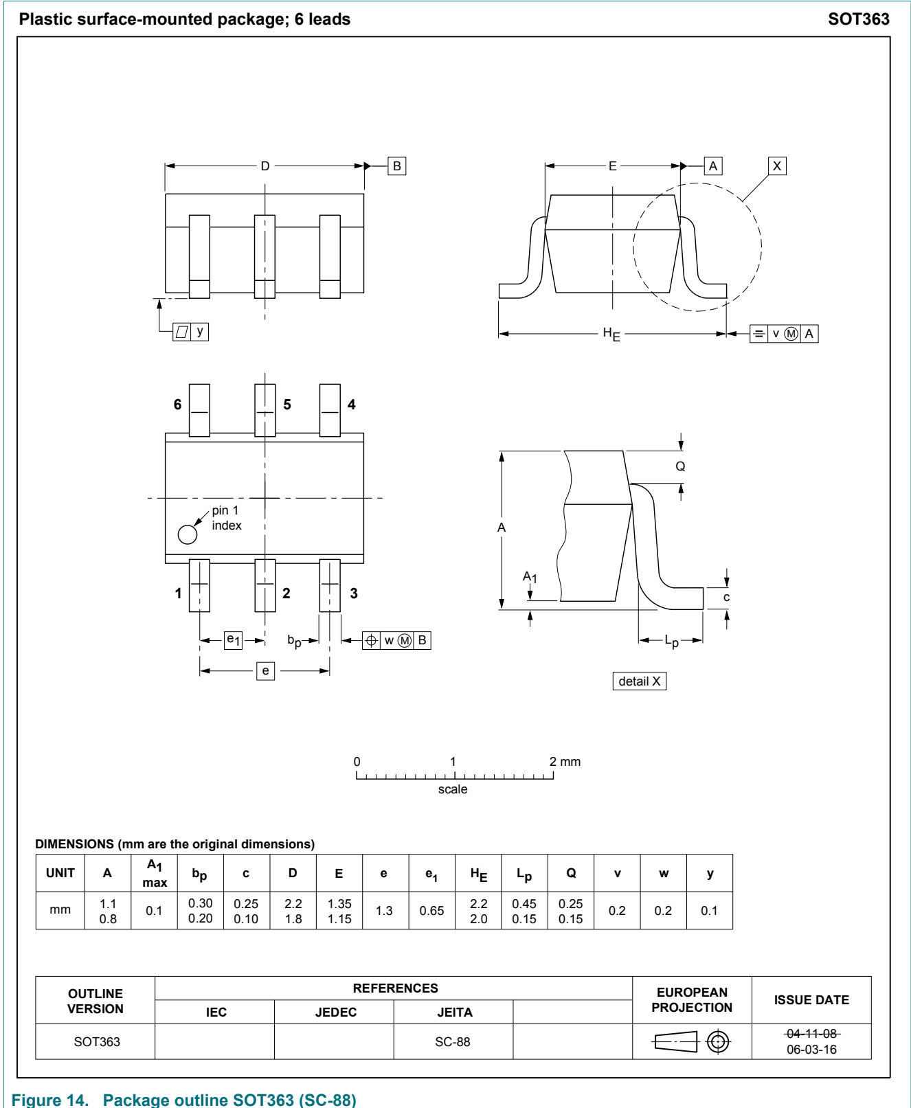
Figure 14. Package outline SOT363 (SC-88)
