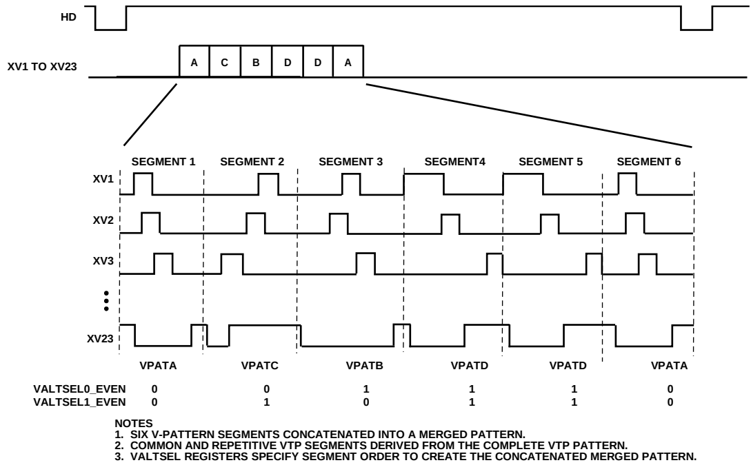
Figure 49. Example of Special V-Sequence Alternation Mode Using VALTSEL Registers to Specify Segment Order
