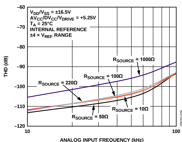
Figure 14. AD7656 THD vs. Input Frequency for Various Source Impedances, ±4 x VREF Range
