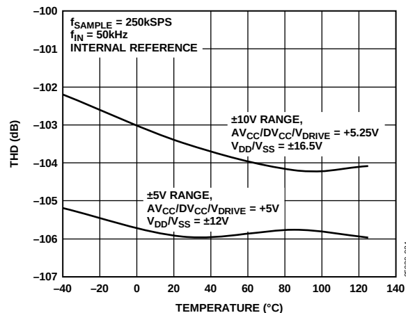
Figure 21. AD7656 THD vs. Temperature
