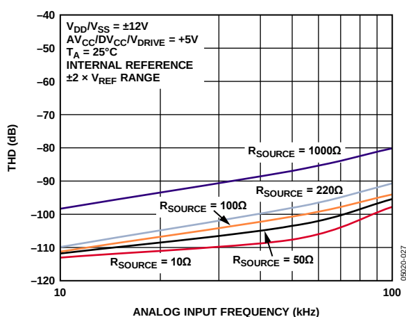
Figure 15. AD7656 THD vs. Input Frequency for Various Source Impedances, ±2 x VREF Range
