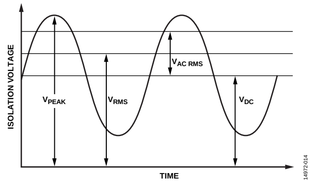
Figure 34. Critical Voltage Example
