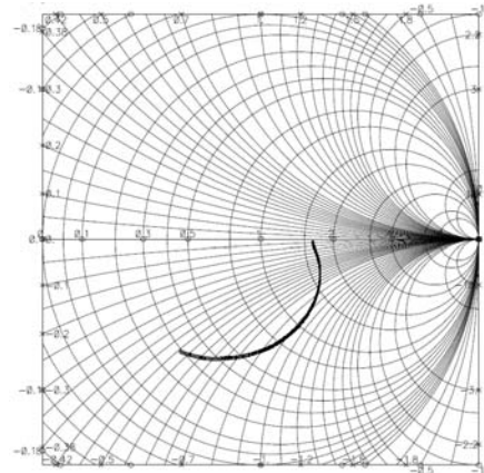
FIGURE 10. SMITH CHART OF S11
