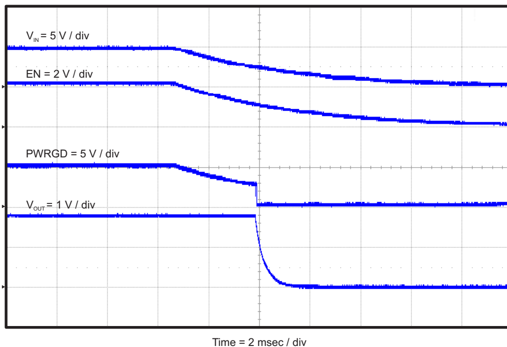
Figure 11. TPS54719EVM-152 Shutdown Relative to V_{IN}
