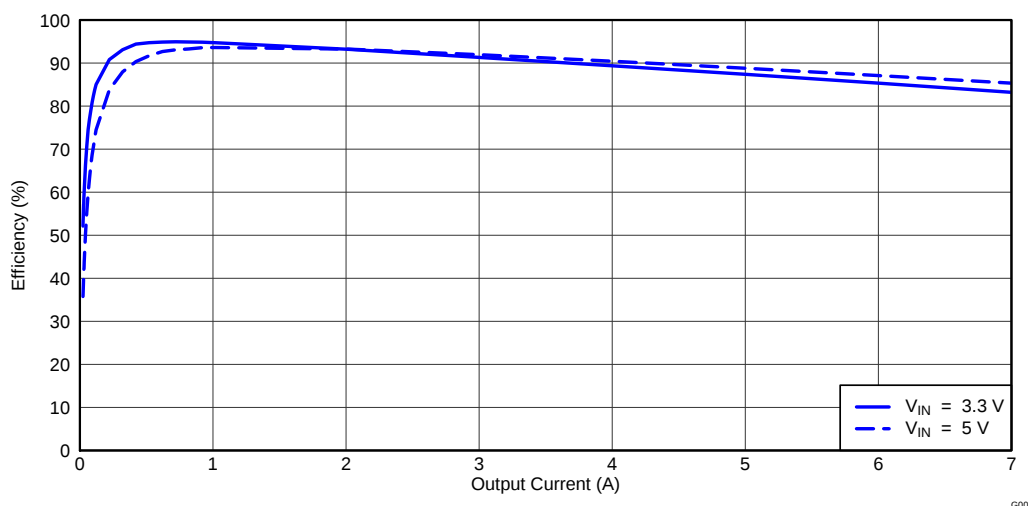
Figure 1. TPS54719EVM-152 Efficiency
