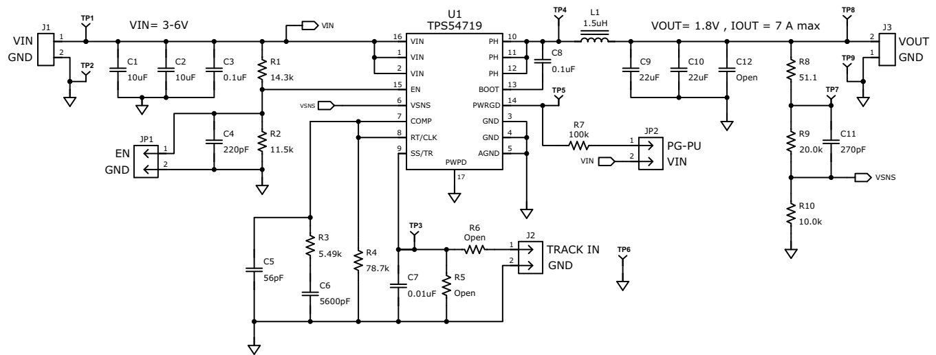
Figure 18. TPS54719EVM-152 Schematic
