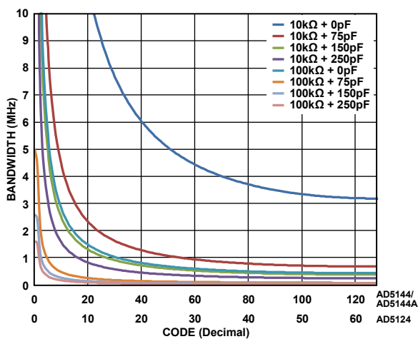
Figure 32. Maximum Bandwidth vs. Code vs. Net Capacitance
