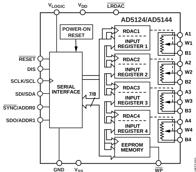
Figure 1. AD5124/AD5144 24-Lead LFCSP
